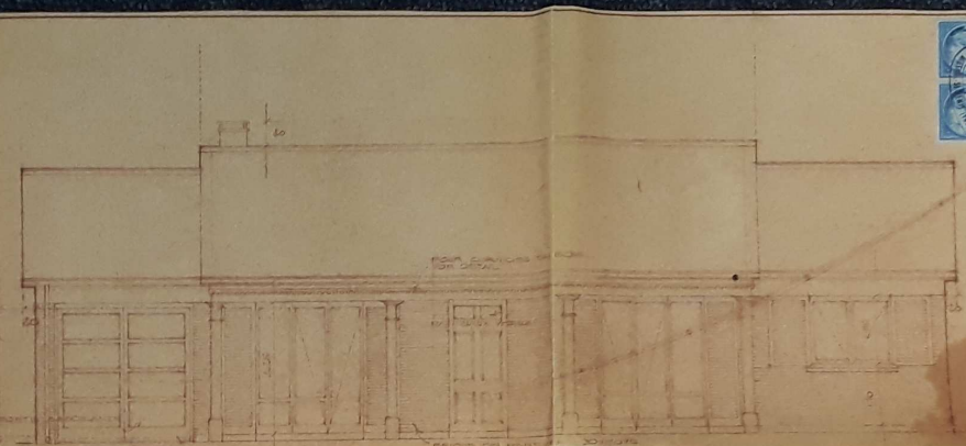
FACADE COTE SUD
